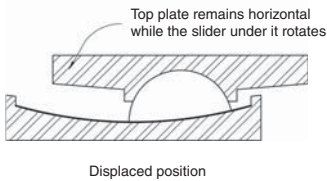
▲ 14.4 A section through a Friction Pendulum™ bearing.
