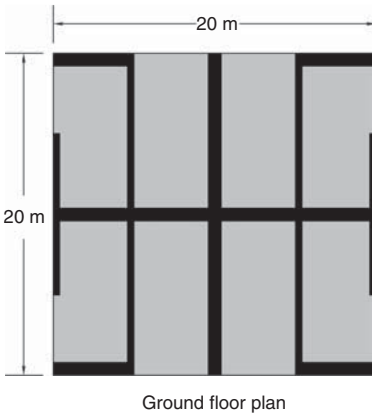
▲ 5.18 Plan of a four-storey confined masonry wall and concrete floor building in the most seismically active zone of Indonesia. The significant lengths and thicknesses of walls drawn to scale are required to satisfy structural requirements. All walls are constructed from brick masonry and are not penetrated.
