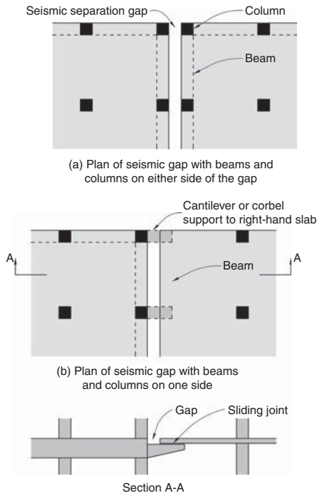
▲ 8.29 Two methods of supporting flooring at a seismic separation gap.
