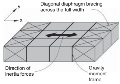
▲ 4.9 Braced diaphragm and cross-bracing for x direction forces.
