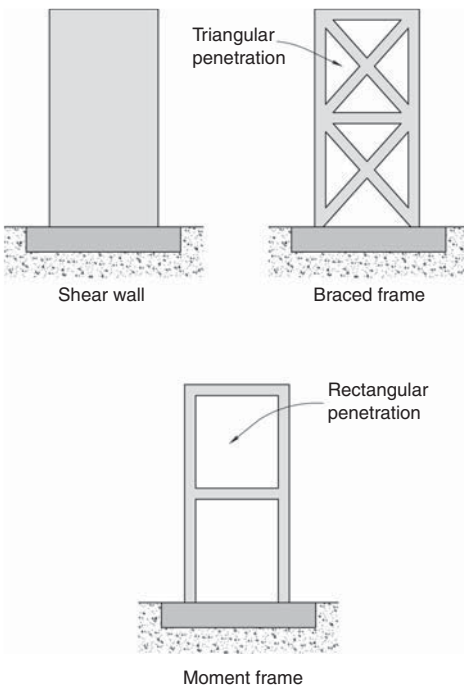
▲ 5.4 Penetrations of a shear wall lead to braced or moment frame systems.
