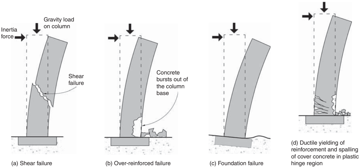
▲ 3.12 Four potential types of failure for a cantilever column. The only ductile and desirable overload mechanism (d) occurs if the other three are suppressed by making them stronger than the force to cause (d).
