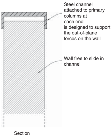
▲ 10.17 Alternative support to a partial-height infill wall. Depending on the wall height and the distance between primary columns the steel channel might require strengthening with welded-on plates.
