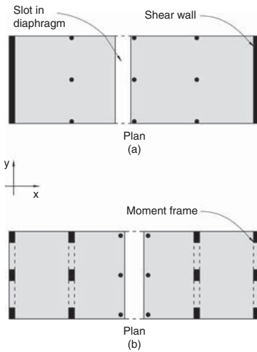
▲ 8.17 A diaphragm slotted near the middle leads to the formation of two separated structures (a). To avoid serious torsional eccentricities, the shear walls are substituted by moment frames (b). The torsional configuration of each structure can be improved if the inner two frames are moved closer to the gap. (X direction structure not shown.)
