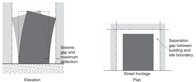
▲ 8.24 Seismic drifts and required separations in elevation and plan to avoid pounding.
