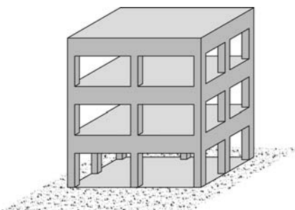
▲ 9.4 A weak column-strong beam structure develops a soft storey at ground level once columns are damaged.
