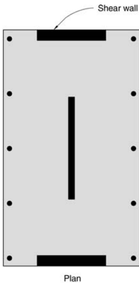
▲ 8.4 Structure located close to the CoR is less effective at resisting torsion.
