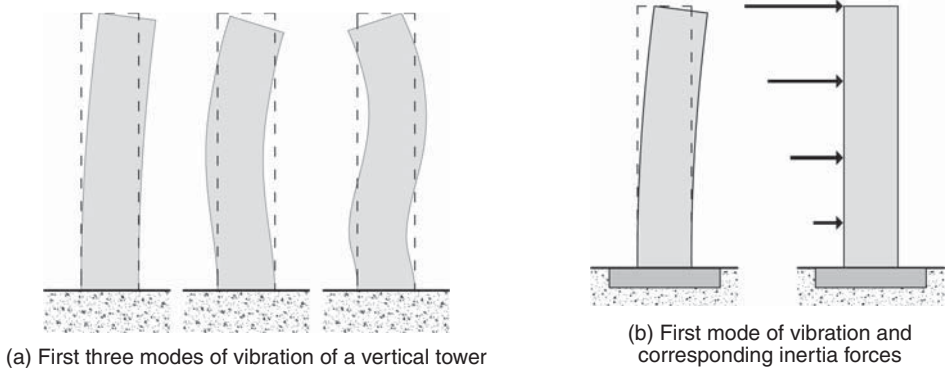
▲ 2.6 The deflected shapes of the first three modes of vibration (a) and the first mode of vibration as the source of most inertia force (b).
