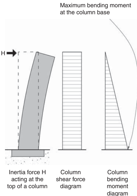
▲ 3.11 The inertia force deflects the column and produces column shear force and bending moment diagrams (The bending moment is drawn on the compression-side of the column rather than the tension-side as is customary in some countries).
