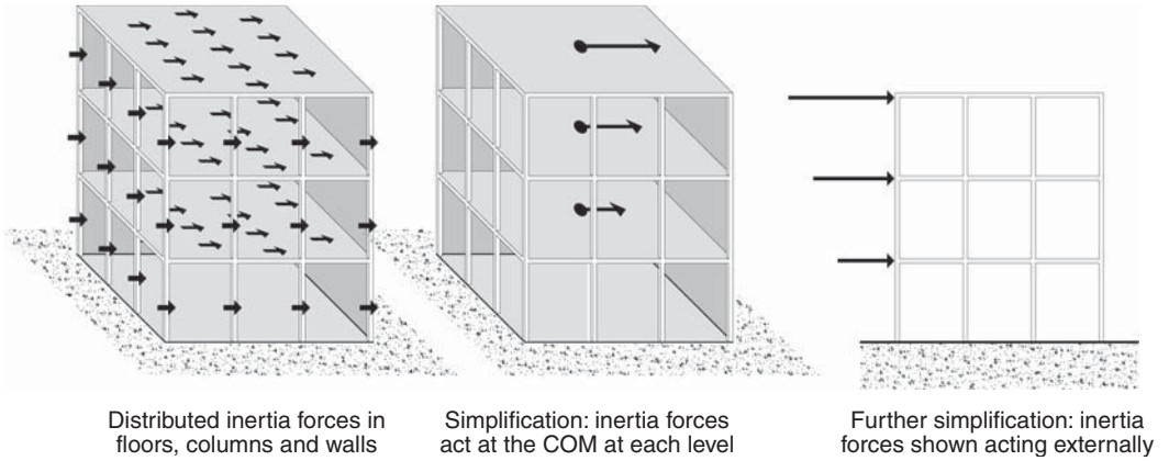
▲ 2.3 Increasing simplification of how inertia forces on a building are expressed graphically.
