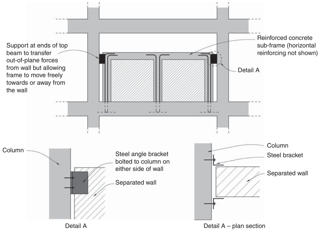
▲ 10.15 The separation of a partial-height unreinforced masonry infill wall.
