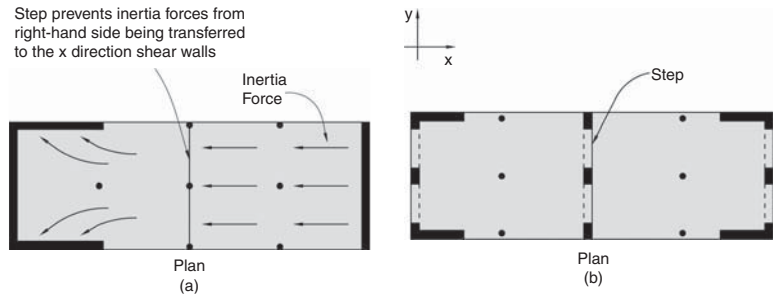
▲ 8.20 The structural difficulty posed by the diaphragm step (a) is solved by increasing the number of shear walls effective in the x direction to four and connecting two to each diaphragm section (b). Moment frames replace y direction shear walls to avoid a mixed system once a moment frame is introduced along the step. Had a shear wall been introduced along the step, the original shear walls in the y direction could have remained.
