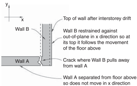
(a) Unseparated corner-interstorey drift in x direction
