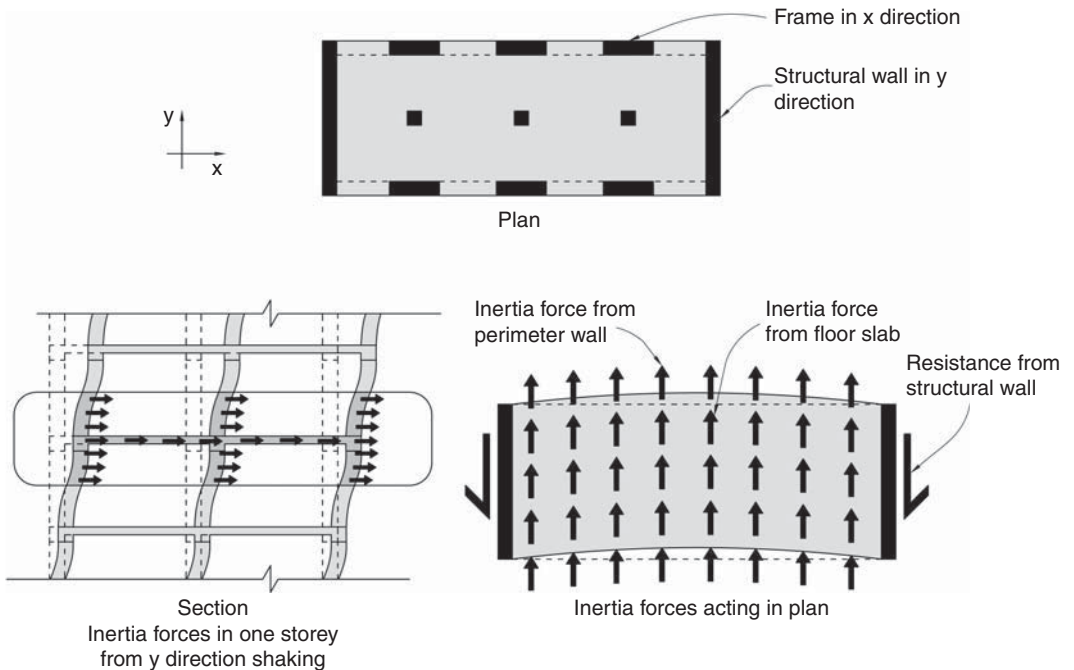
▲ 4.1 Inertia forces within a multi-storey building shown in plan and section.
