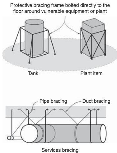
▲ 11.24 Examples of mechanical plant restraints.
