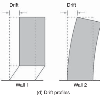
▲ 9.16 A discontinuous wall and its torsion-inducing influence on a building.
