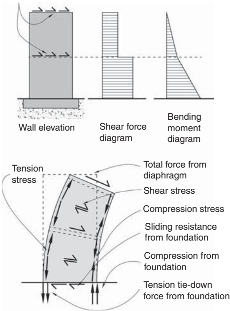
▲ 5.3 Forces acting on and within a shear wall.
