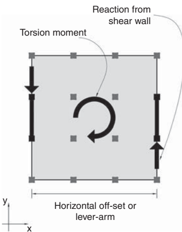
▲ 5.5 Seismic force in the y direction is resisted by two shear walls. Because of the off-set or lever-arm between them they also resist torsion. Structure acting in the x direction is not shown.
