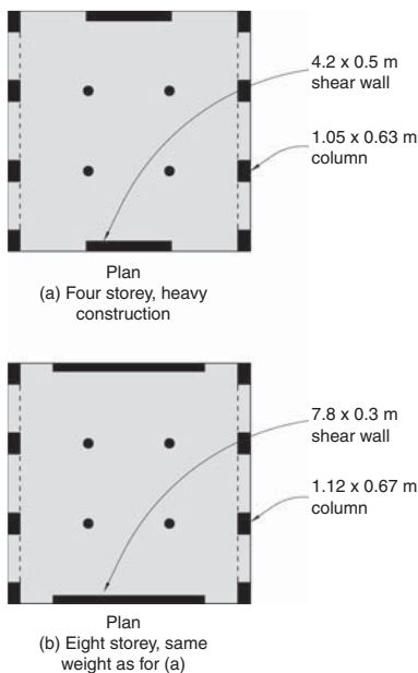
▲ 6.13 Ground floor plans of a four and eight-storey building of the same weight (gravity structure not shown. Drawn to scale).
