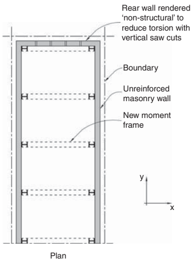
▲ 12.7 Y direction seismic forces are resisted by long masonry walls but new moment frames are required to resist x direction forces. Frame columns also provide out-of-plane resistance to the masonry walls.
