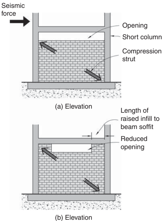
▲ 9.14 Reduction in the width of an opening above a partial-height masonry or concrete infill to prevent a short column failure. The raised lengths of infill enable a compression strut to transfer force directly to the top of the column and avoids the need for the column to bend.
