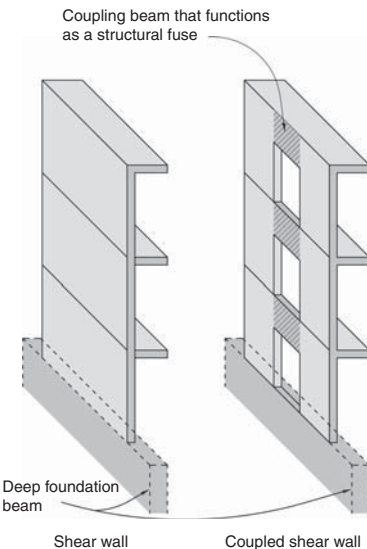
▲ 5.21 Comparison between a shear wall and a coupled shear wall.
