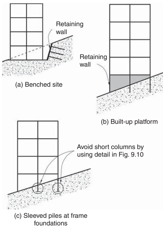
▲ 9.23 Structural configurations for moment frames on sloping sites.
