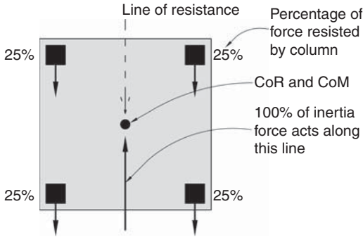
(a) Ground floor plan: identical columns
