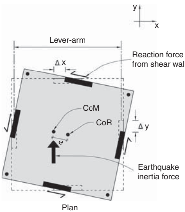
▲ 8.3 A building plan illustrating how vertical structure resists torsion. Most gravity-only structure and the movement of the building in the y direction is not shown.
