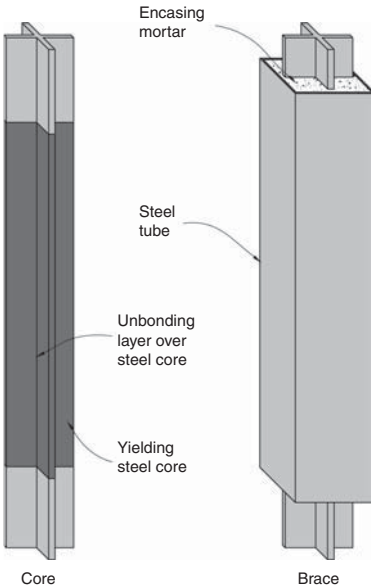
▲ 14.19 Schematic details of a buckling-restrained brace.
