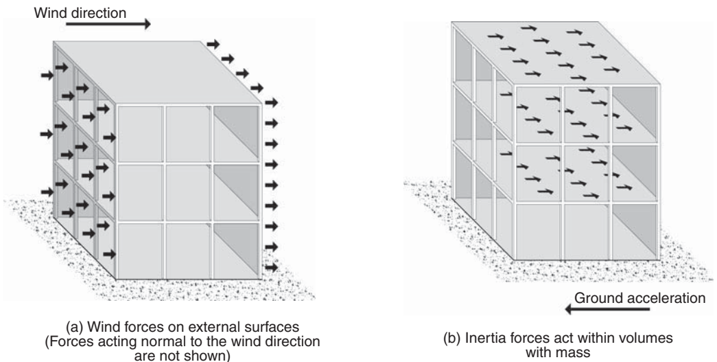
▲ 2.4 Comparison between externally acting wind forces and internal inertia forces.
