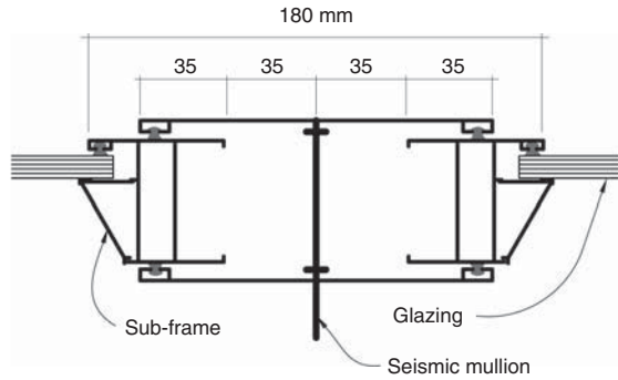
▲ 11.15 An extruded aluminium seismic mullion that allows for \pm 35 mm of movement.
