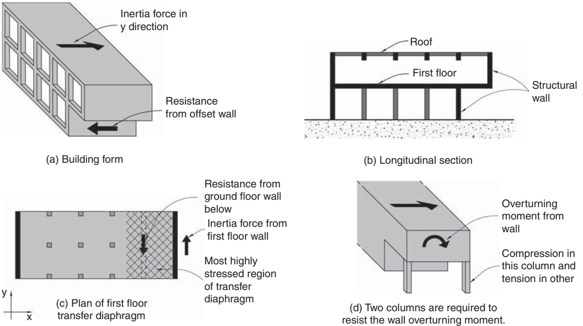
▲ 4.15 A transfer diaphragm provides a force path for horizontal shear forces from the upper wall to the offset ground floor wall.
