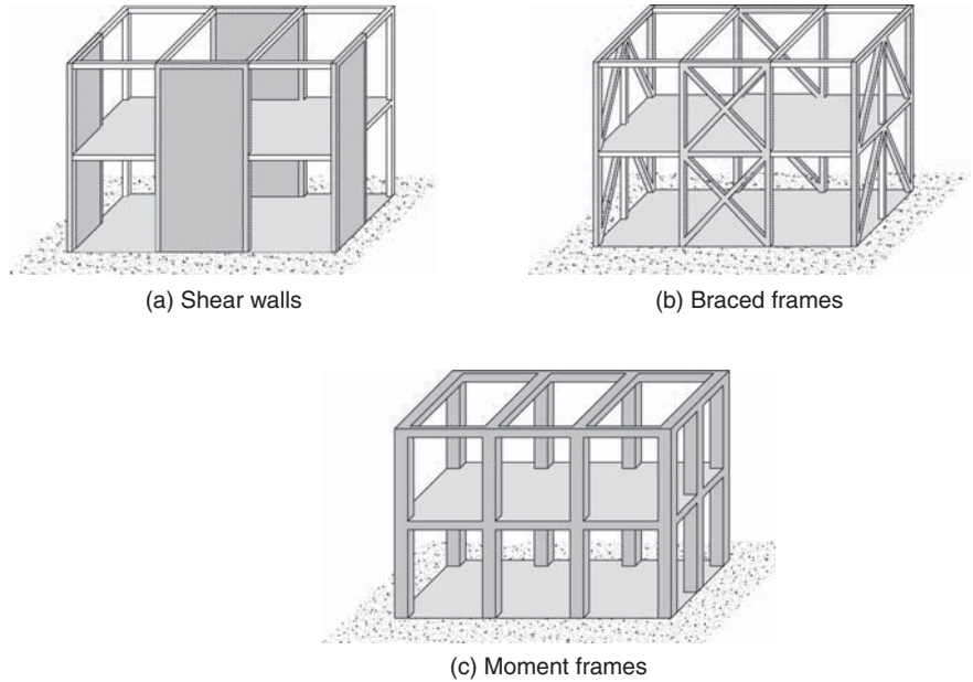
▲ 5.2 The three basic seismic force resisting systems.
