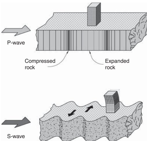
▲ 1.10 Dynamic ground movements caused by the propagation of P- and horizontal S-waves.
