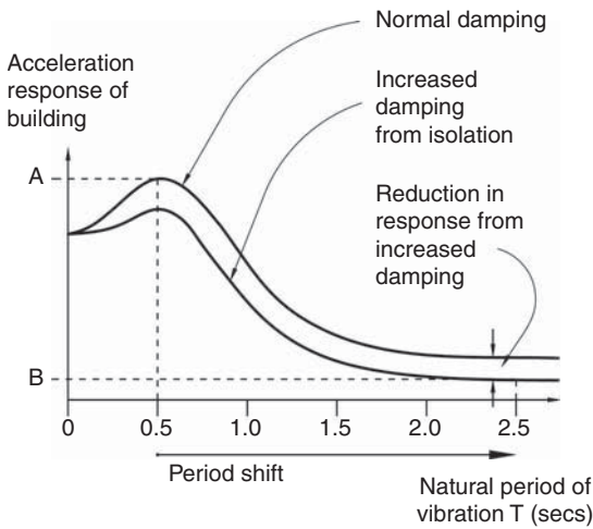
▲ 14.2 A response spectrum showing how the peak acceleration of a fixed-base building, A, is reduced to B by the 'period shift' and increased damping of a seismic isolation system.
