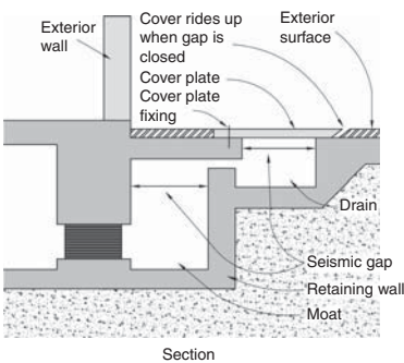
▲ 14.9 Possible section through the perimeter of a seismically isolated building.
