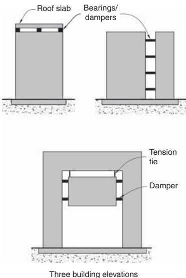
▲ 14.24 Theoretical examples of where discontinuities and dampers are inserted into buildings with the intention of reducing the overall seismic response.
