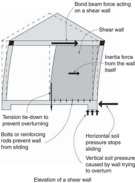
▲ 2.21 Inertia forces and resisting actions on a shear wall.
