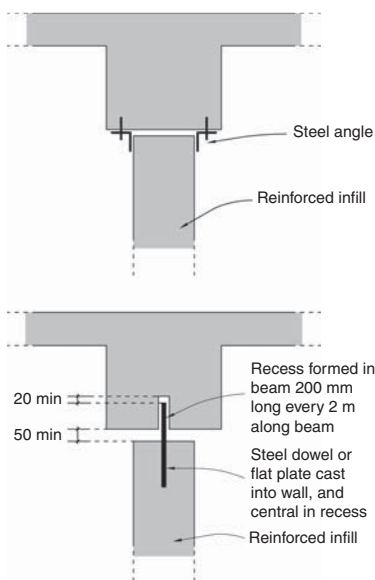
▲ 10.11 Two possible structural details that resist out-of-plane forces yet allow relative movement between an infill wall and structure above.
