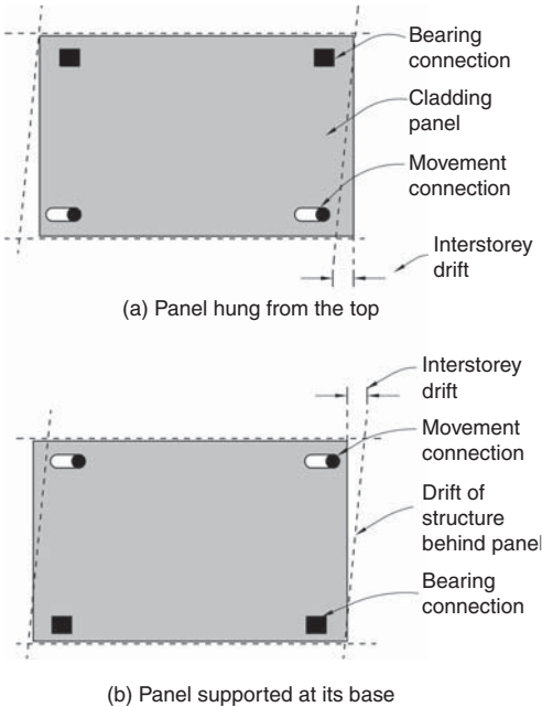
▲ 11.7 Fully separated storey-height panel, top-hung (a) and supported at its base (b).
