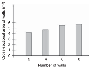
▲ 6.14 The plan area or footprint of seismic resisting structure increases with the number of shear walls. This graph applies for one direction of loading.
