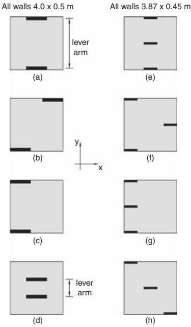
▲ 6.3 Ground floor plans showing different shear wall layout options that provide symmetrical resistance for x direction seismic forces (Y direction and gravity structure not drawn).
