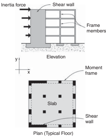
▲ 5.49 An example of a mixed system comprising shear wall and moment frame.
