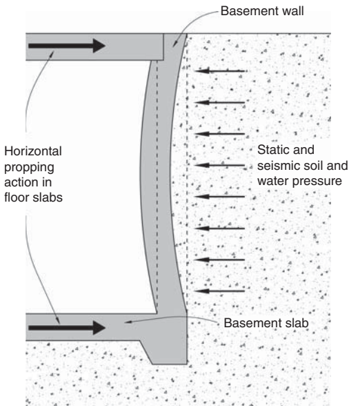
▲ 7.11 A reinforced concrete basement wall propped against horizontal soil pressures by slabs, top and bottom.
