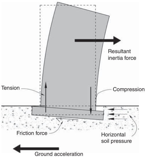
▲ 7.1 Forces acting on a foundation from the superstructure and the ground.
