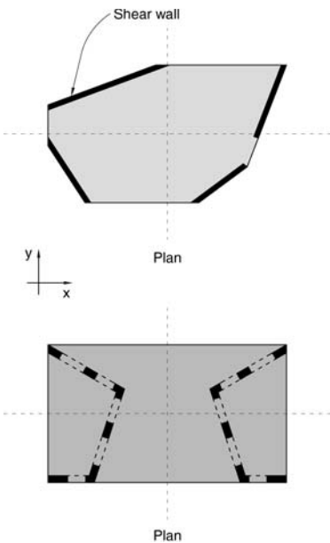
▲ 8.21 Two examples of non-parallel systems. Gravity-only structure not shown.
