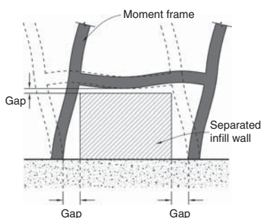
▲ 10.9 Infill wall with separation gaps between infill and columns and beam.
