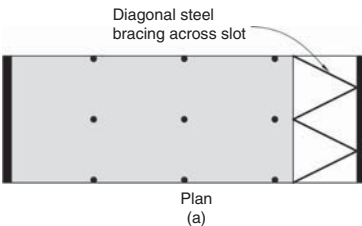
▲ 8.14 A slot in the diaphragm destroys its ability to span between shear walls for y direction forces. ( x direction structure not shown.)
