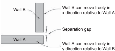
(b) Separated corner detail
