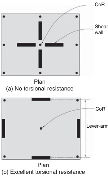
▲ 8.2 Two structural configurations, each with four shear walls, with contrasting abilities to resist torsion.
