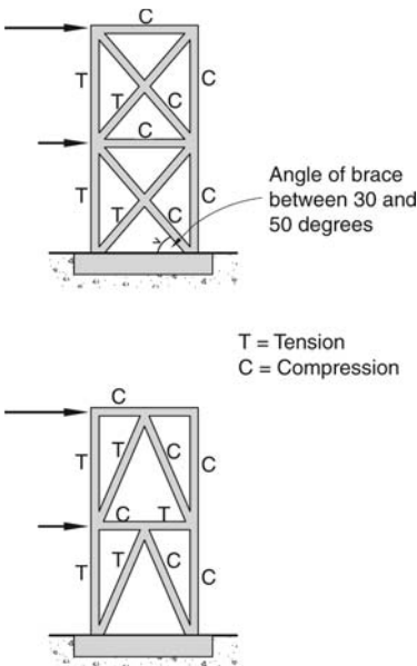
▲ 5.27 Two tension and compression fully triangulated frames. The types of axial force are indicated.
