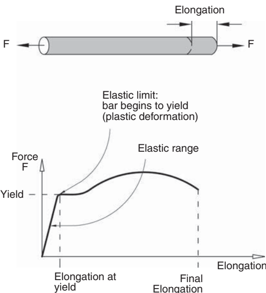
▲ 2.10 A graph of tensile force against elongation of a steel rod.
