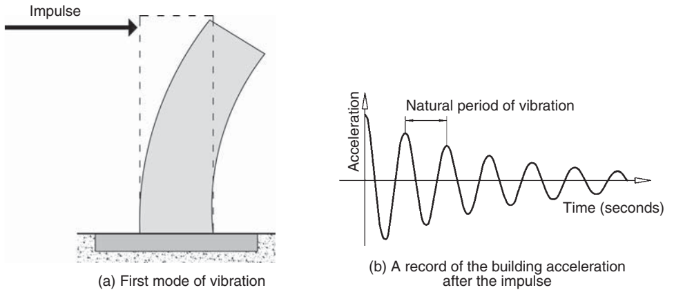
▲ 2.5 A building given an impulsive force (a) and subsequent vibrations at its natural period of vibration (b).
