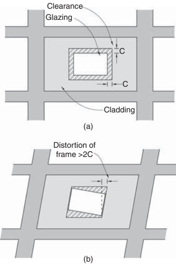
▲ 11.14 A glass windowpane set inside a frame with clearance all around (a). In a distorted frame the glass has slid and rotated relative to the base of the frame (b). Further distortion will lead to glazing damage.
