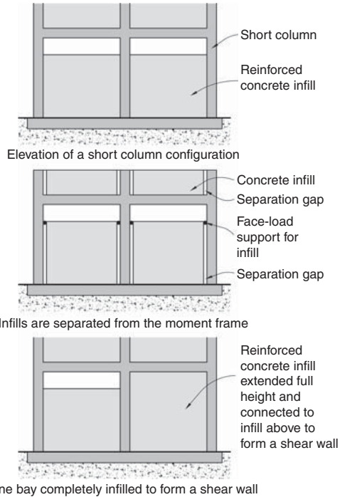
▲ 9.15 Methods to avoid a short column configuration with reinforced concrete infills.
