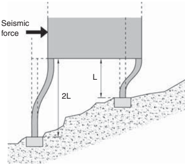
▲ 9.9 Two unequal height columns resisting seismic force.
