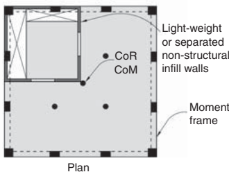
(b) Eccentric core, but regular horizontal configuration
