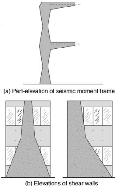
▲ 17.3 Haunched members of a moment frame (a) and tapered shear walls (b) reflect their seismic bending moment diagrams.
