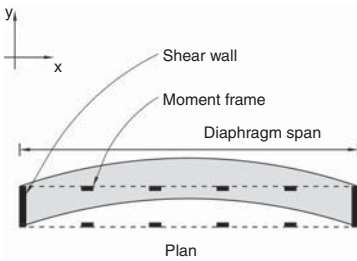
(a) Diaphragm deflecting under y direction inertia forces. Since its span is excessive for its depth it may be too weak or flexible
