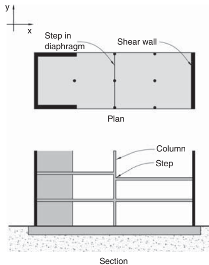
▲ 8.18 A stepped diaphragm.
