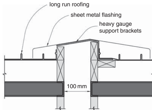
Section detail at roof separation
