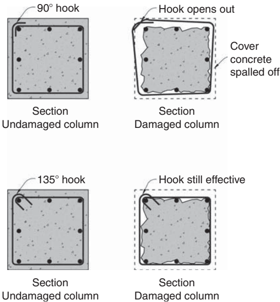
▲ 12.5 Incorrectly bent column (and beam) ties are dangerous. During an earthquake their hooks open out and the ties lose all their effectiveness.
