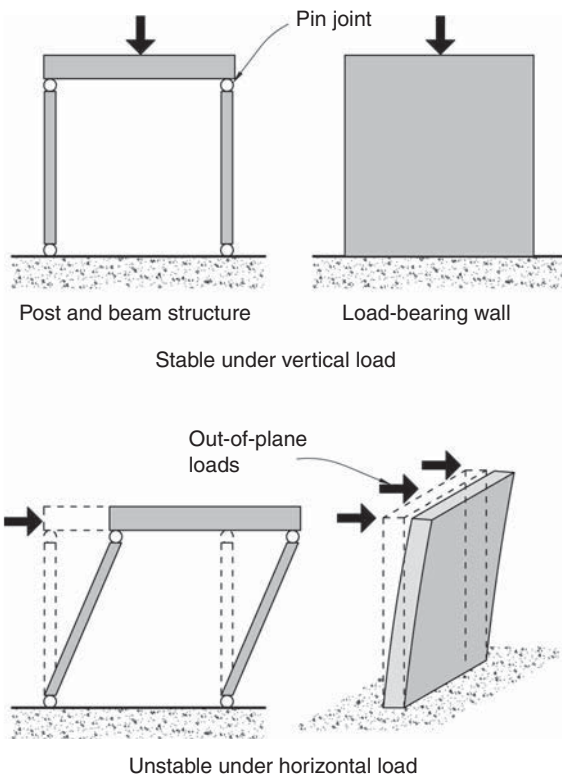
▲ 5.1 Instability of two gravity force resisting structures against horizontal forces.
