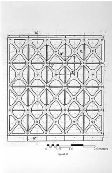
▲ 12.2 A proposed perforated steel shear wall adds a layer of architectural richness to an interior wall of a historic unreinforced masonry building, Wellington.
