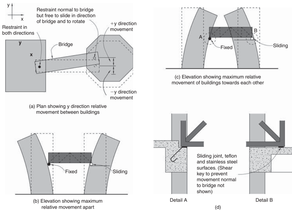
▲ 8.31 The relative drifts between two separated buildings (a) to (c) and generic bridge seating details (d).
