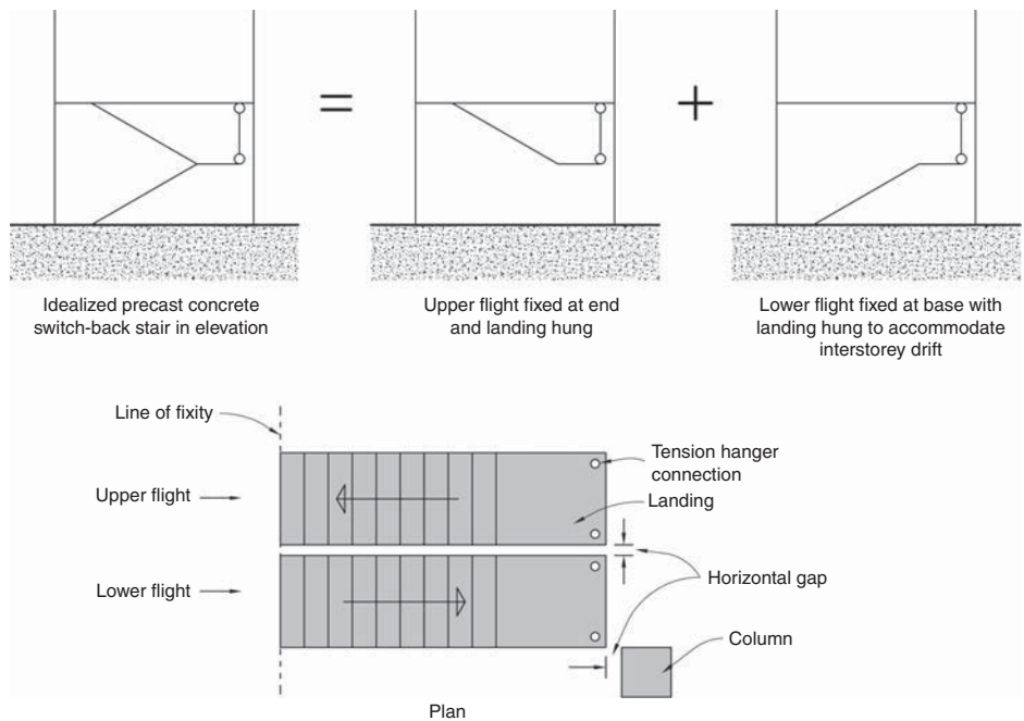
▲ 10.23 Idealized elevations and plan showing a method of separating a switch-back stair from the structure.
