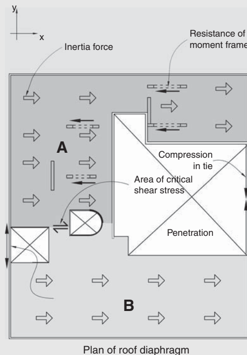
▲ 6.27 Inertia forces acting in the x direction; the resistance from the proposed structure and the axial forces in the two perimeter tie members.
