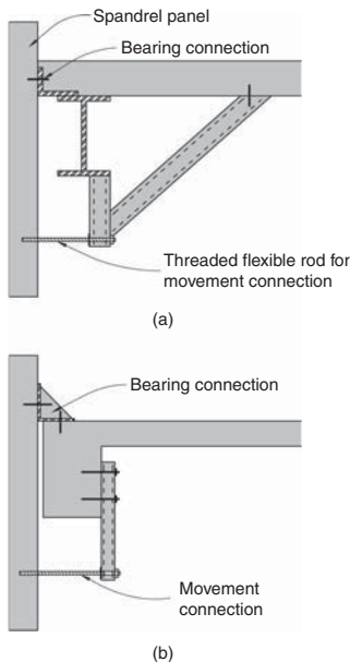
▲ 11.12 Spandrel panel bearing and movement connection details for a steel frame (a) and a reinforced concrete frame (b).
