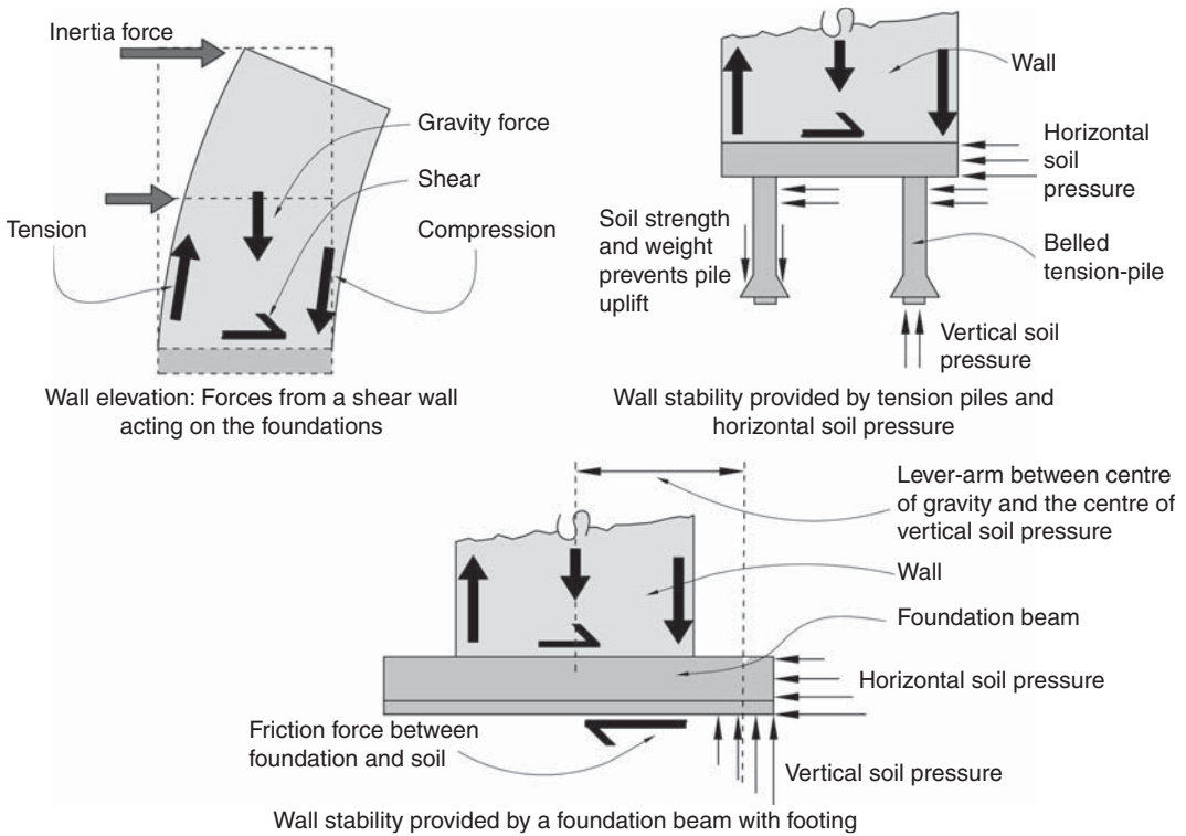
▲ 5.9 How foundations resist overturning moments and shear forces from a vertical structure, in this case a shear wall.
