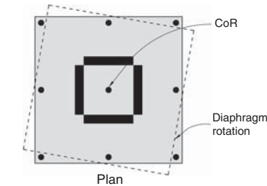
(b) Diaphragm rotation increases where inner walls alone resist torsion
