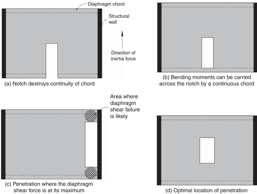
▲ 4.14 Diaphragm penetrations in various locations.
