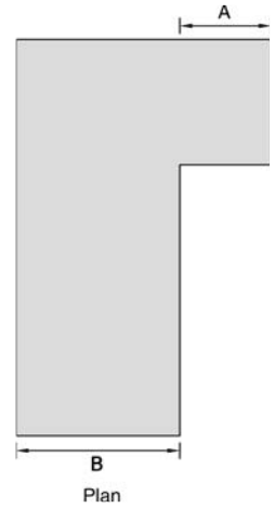
▲ 8.12 A typical definition of an irregular re-entrant configuration is where A > 0.15B .
