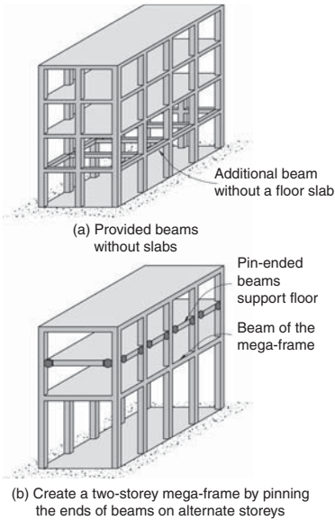
▲ 9.7 Two methods of avoiding a soft storey where one storey is higher than others.
