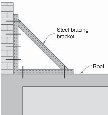
(b) Elevation Steel bracket
