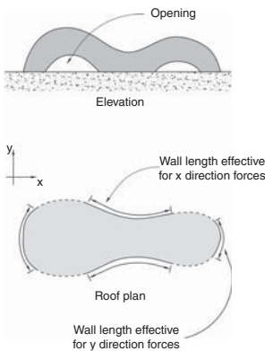
▲ 6.18 Bracing lengths for an irregular shell structure.
