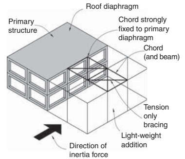
▲ 4.11 A secondary diaphragm cantilevers horizontally from the primary structure to avoid vertical end-wall cross bracing.
