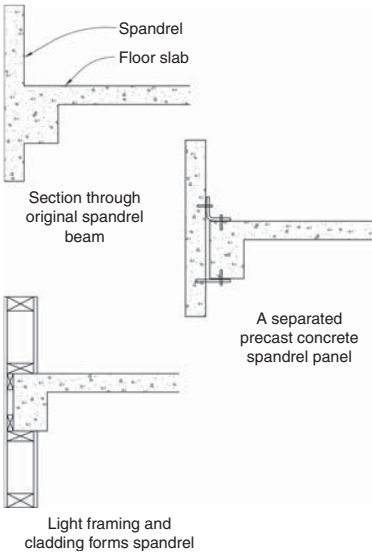
▲ 9.5 Options for non-structural spandrel panels.
