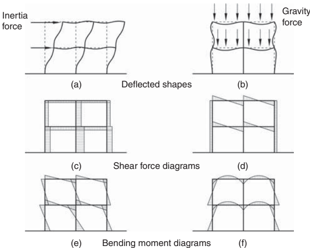
▲ 5.32 Comparison between a horizontally loaded moment frame and a frame supporting gravity forces.
