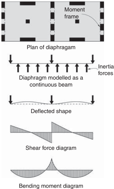
▲ 4.5 A continuous two-span diaphragm.
