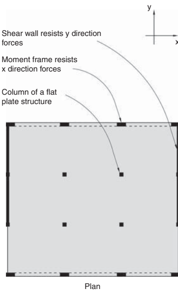
▲ 5.38 Plan of a flat plate gravity-resisting structure provided with seismic resistance by a pair of shear walls and moment frames.
