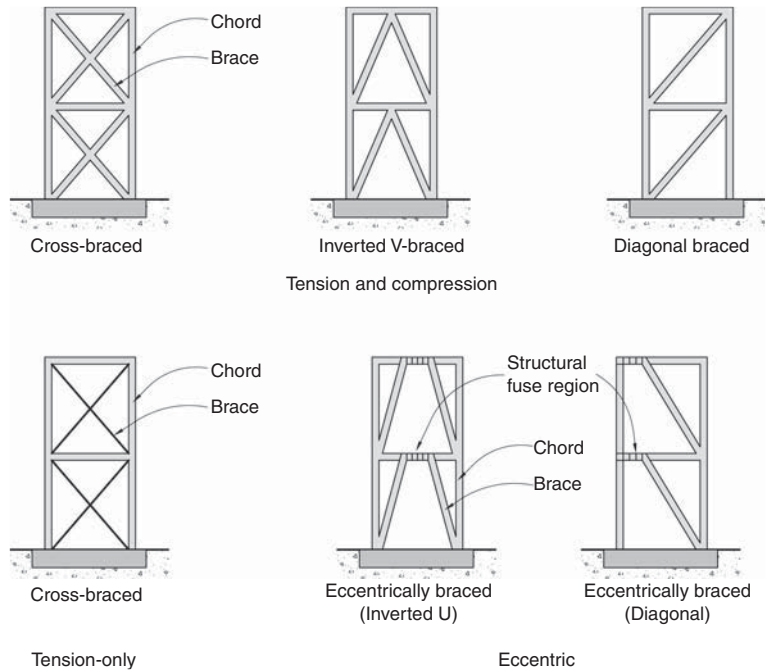
▲ 5.23 Common types of braced frames.
