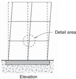
▲ 14.21 Damage avoidance precast concrete shear wall system.
