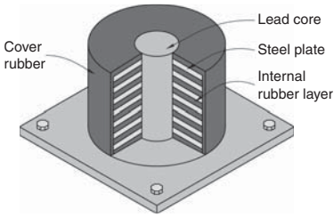
▲ 14.3 A cut-away view of a lead-rubber bearing.
