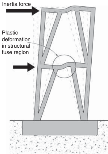
▲ 5.25 The deformation of an eccentrically braced frame showing the distortion of the structural fuses.
