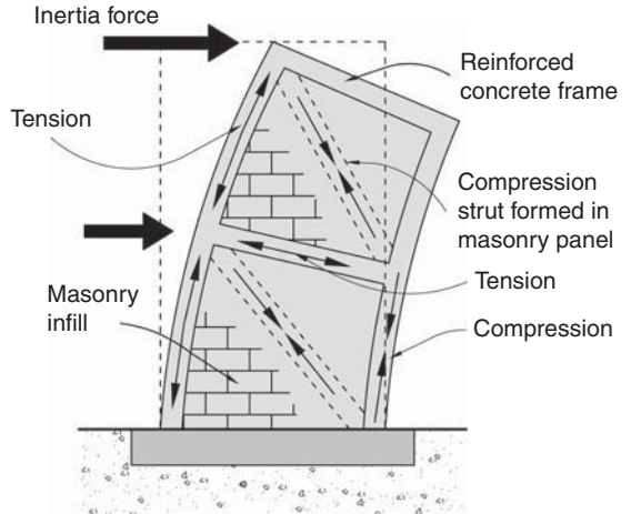
Elevation of a confined masonry wall showing internal 'truss action' forces
