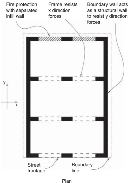
▲ 3.9 Plan of a building whose structural walls on the boundary provide excess seismic strength in the y direction. Frames resist x direction forces.
