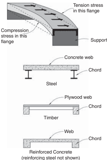
▲ 4.4 A steel channel beam analogous to a diaphragm and cross-sections through diaphragms of different materials.
