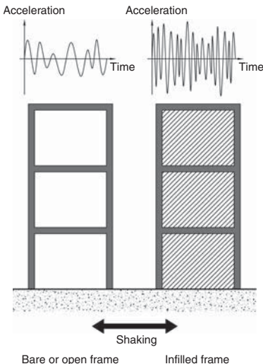
▲ 10.3 A comparison of roof-top accelerations of a bare or open frame with an infilled frame. Note the shorter periods of vibration and higher accelerations of the infill frame.
