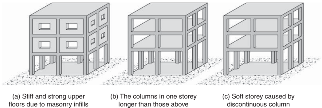
▲ 9.3 Examples of soft storey configurations.
