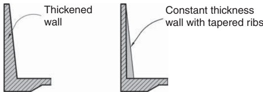
(b) Sections through two wall options where the wall resists out-of-plane inertia forces by cantilever action
