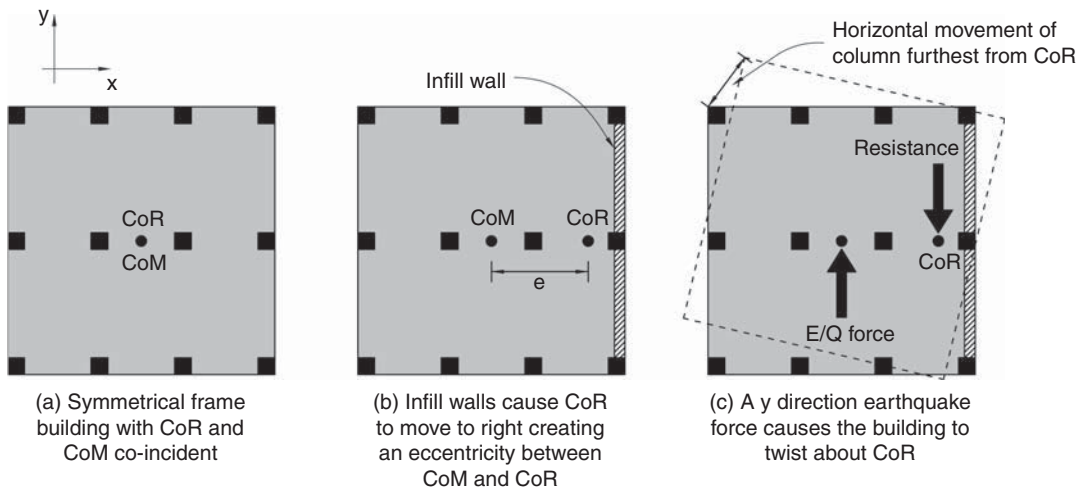
▲ 10.8 Asymmetrically placed infill walls cause building torsion that damages columns distant from the CoR.
