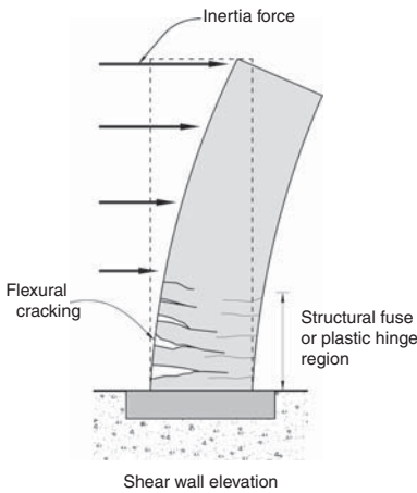
▲ 5.19 Structural fuse region at the base of a ductile shear wall. The vertical reinforcing yields and absorbs earthquake energy.
