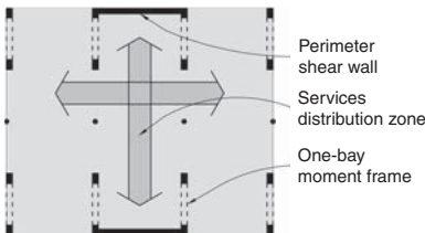
(a) One-way, one-bay frames allow distribution of under-floor services
