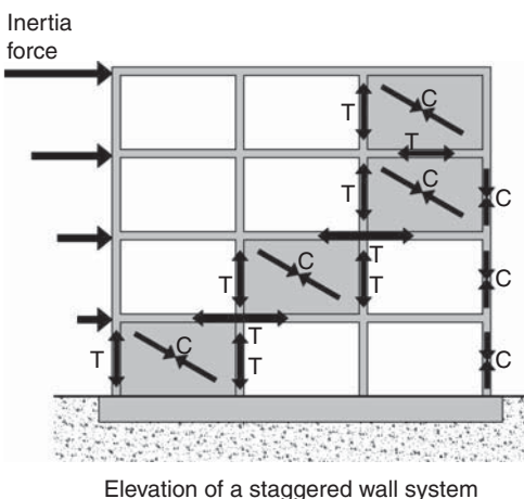
▲ 9.20 The indirect force paths of a staggered-wall system.
