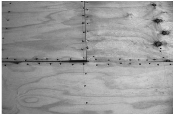
▲ 5.20 The plywood web of a wood shear wall is fixed to framing with closely-spaced nails that transfer forces between sheets and yield in bending to act as structural fuses. School building, Wellington.
