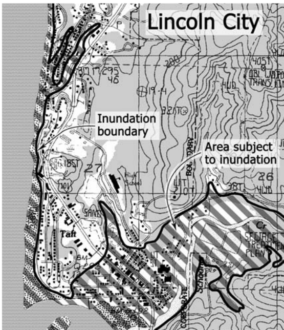
▲ 15.4 An inundation map for a section of the US West Coast for a tsunami caused by a magnitude 8.8 undersea earthquake. (Adapted from a map, State of Oregon, Dept. of Geology and Mineral Industries).
