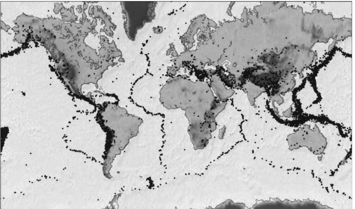
▲ 1.7 Geographic distribution of earthquakes. Each dot on the map marks the location of a magnitude 4 or greater earthquake recorded over a period of five years. (Reproduced with permission from IRIS Consortium).
