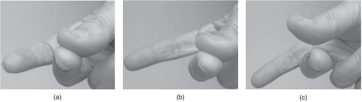
▲ 1.4 Experience the build-up of tectonic strain and energy release by snapping your fingers. Apply pressure normal to your finger and thumb (a), next apply sideways force (b), and then feel the sudden snapping when that force exceeds the friction between thumb and finger (c).
