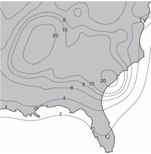
▲ 1.8 A map of an area of the U.S.A. showing horizontal acceleration contours expressed as a percentage of the acceleration due to gravity. The values, applicable to low-rise buildings founded on rock, have a 10% probability of exceedence in 50 years.
