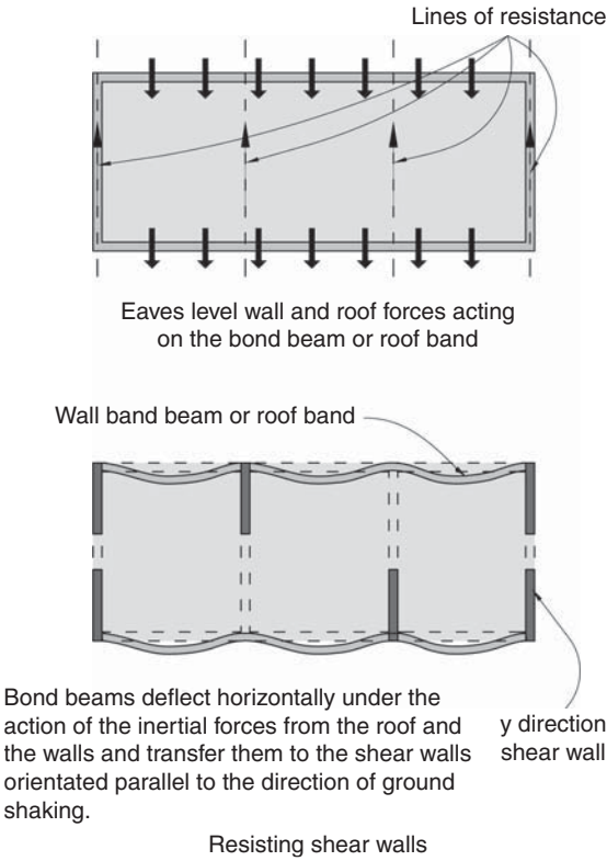
▲ 2.19 Bond beams or roof bands distribute inertia forces at eaves level to shear walls parallel to the y direction.
