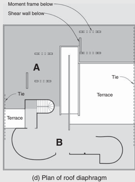
▲ 6.26 Simplified floor and roof plans of the Villa Savoye showing the proposed seismic structure if rebuilt in a seismically active area.
