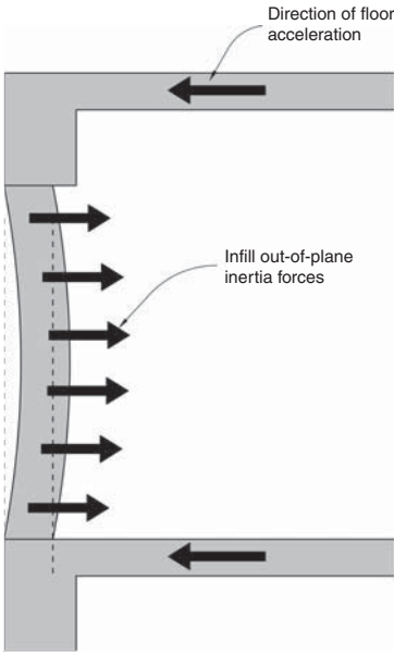
▲ 10.7 A section through two floors and an infill wall. Out-of-plane forces act on the infill which spans vertically between floors.
