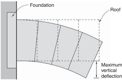
Elevation of a shear wall building
