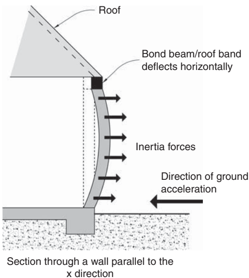
▲ 2.18 Effects of out-of-plane inertia forces on a wall.
