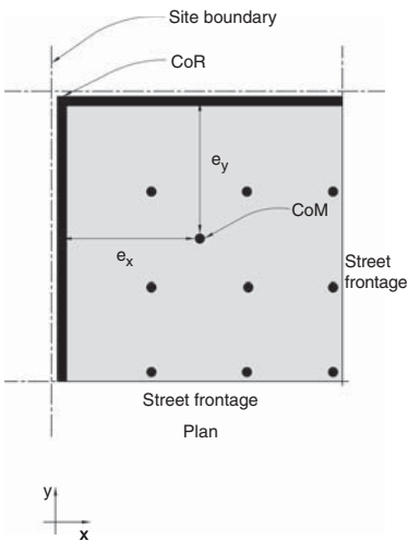
▲ 8.6 Poor configuration of a typical corner building with shear walls as boundary walls.
