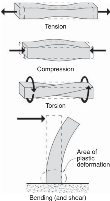
▲ 2.11 Different structural actions causing ductile deformations in structural elements.
