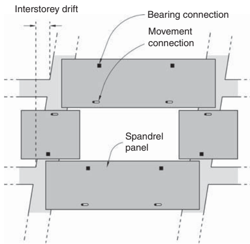
▲ 11.11 One approach to isolating spandrel and column panels from the interstorey drifts of a structural frame.
