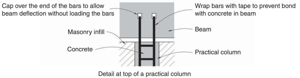
▲ 10.14 Separated unreinforced masonry infill wall with 'practical columns' providing out-of-plane strength.
