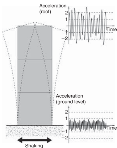
▲ 10.1 Shaking at ground level is amplified up the height of a building.
