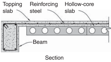
▲ 4.6 Part section through a precast concrete and topping slab diaphragm.
