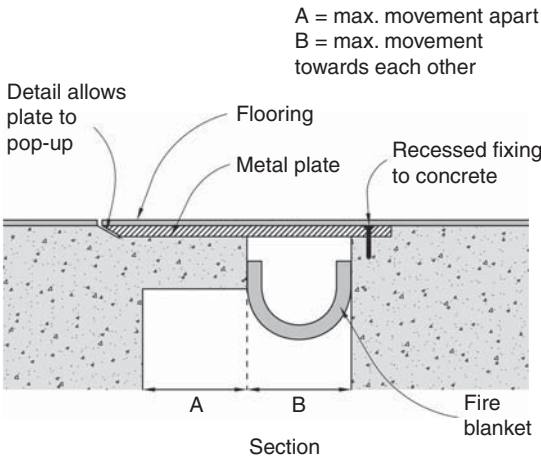
▲ 8.27 A section through a generic floor level seismic gap. Dimension 'A' can be reduced if damage caused by the plate sliding off its left-hand seating is acceptable during smaller relative drifts.
