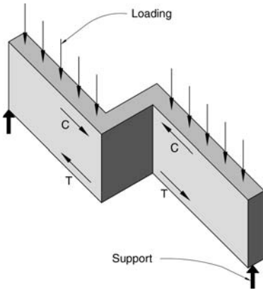
▲ 8.19 A kinked beam showing internal compression and tension forces that can not be achieved. The beam is structurally unsound.
