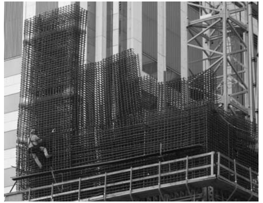
▲ 5.11 Reinforcing steel for cast-in-place concrete shear walls. High-rise office building, San Francisco.
