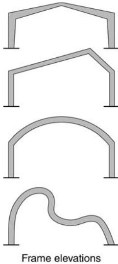
Frame elevations
