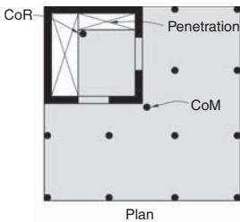
(a) Undesirable configuration caused by an eccentric structural core
