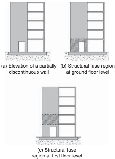
▲ 9.19 A partially discontinuous wall and options for the location of its structural fuse or plastic hinge region.
