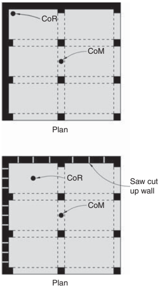
▲ 12.6 By weakening the structural walls, the centre of rigidity (CoR) is brought closer to the centre of mass (CoM), reducing torsional eccentricity.
