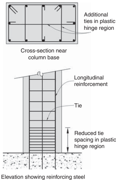
▲ 3.14 Additional reinforcing steel to confine the concrete in the fuse or plastic hinge region of a column.
