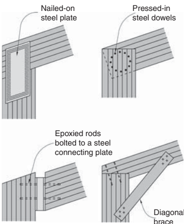
▲ 5.40 Methods of forming rigid joints in (glue-laminated) wood moment frames.
