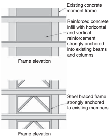
▲ 12.8 Transformation of a concrete moment frame into a shear wall and braced frame.
