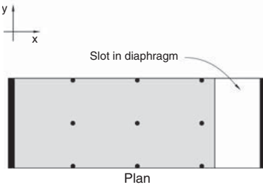
▲ 8.14 A slot in the diaphragm destroys its ability to span between shear walls for y direction forces. ( x direction structure not shown.)
