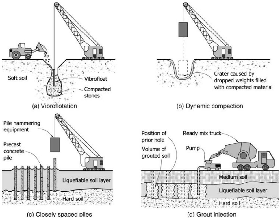
▲ 7.4 Common methods of ground improvement to prevent liquefaction.
