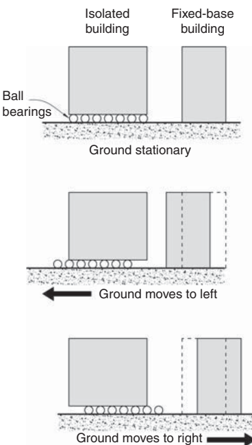
▲ 14.1 Relative movement between the ground and a perfectly isolated building on ball bearings, and a fixed-base (conventional) building.
