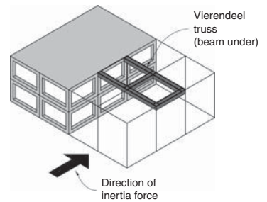
▲ 4.12 A vierendeel truss as a cantilevered diaphragm.
