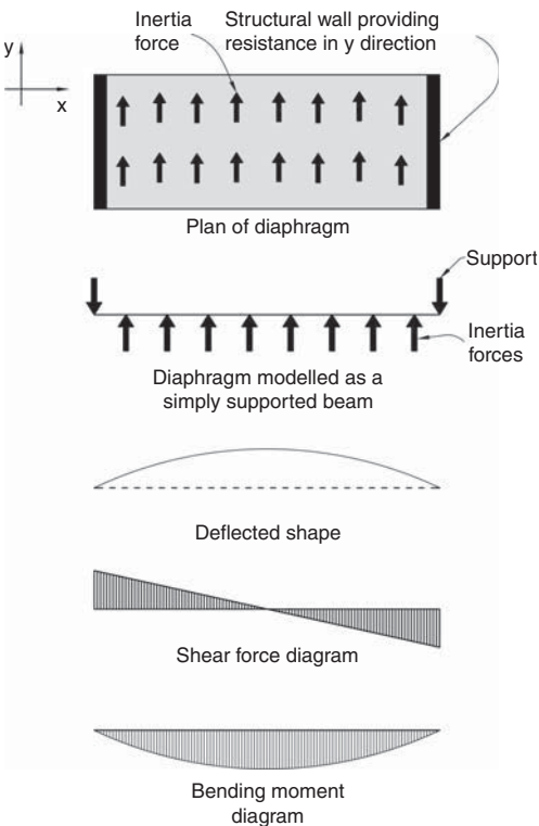
▲ 4.3 A diaphragm as a simply-supported beam.
