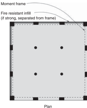
▲ 8.7 An improved horizontal configuration for a corner building. Horizontal forces are resisted by symmetrical moment frames.
