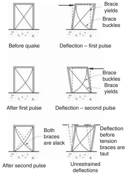
▲ 5.30 Under cyclic loading, yielding of tension-only braces result in a floppy structure.
