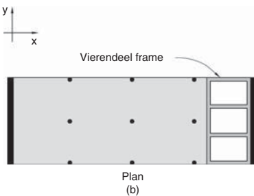
▲ 8.15 Plans of two diaphragms where structural integrity across a slot is restored by steel bracing and frame-action.
