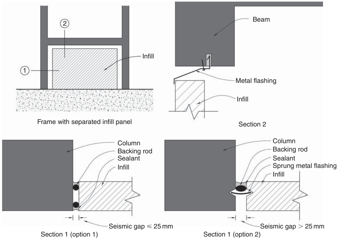
▲ 10.10 Some typical architectural details of separation gaps between an infill wall and frame.
