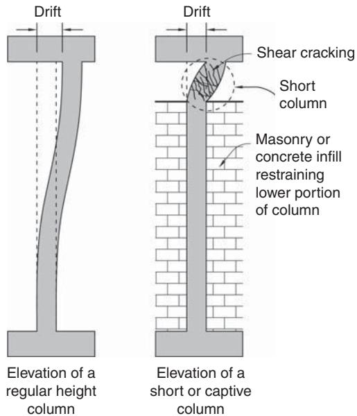
▲ 9.11 Comparison between a regular and a short column subject to horizontal drift.
