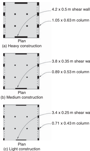
▲ 6.12 Ground floor plans of a four-storey building showing how structural dimensions change for different construction weights (drawn to scale).
