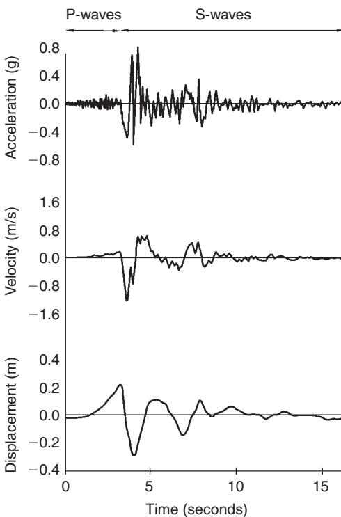
▲ 1.12 North-south components of acceleration, velocity and displacement histories from Sylmar, California, during the 1994 Northridge earthquake. (Adapted from Norton et al. , 1994).
