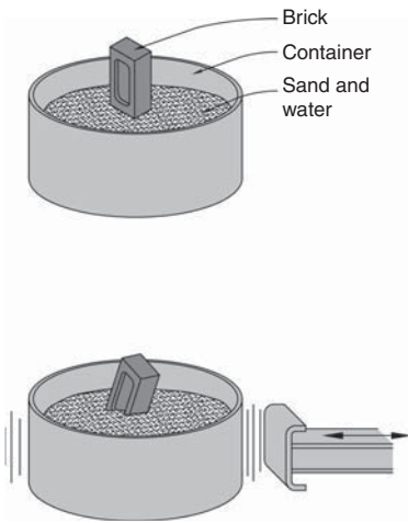
▲ 7.2 A simple demonstration of liquefaction.
