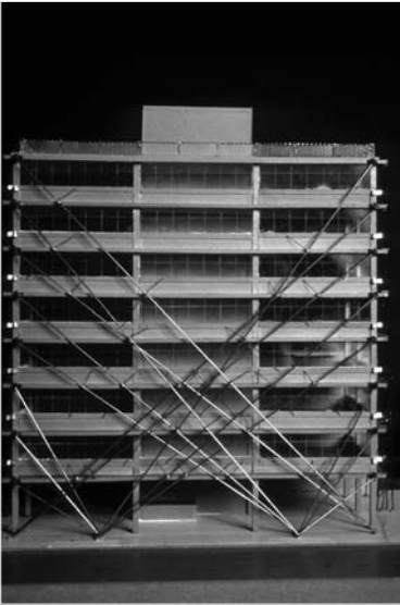
▲ 12.3 A proposed retrofit scheme for a 1960s lift-slab commercial building, Wellington. The scheme references temporary propping to earthquake damaged buildings.
