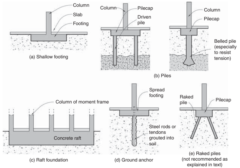
▲ 7.8 Common foundation types for seismic resistance.
