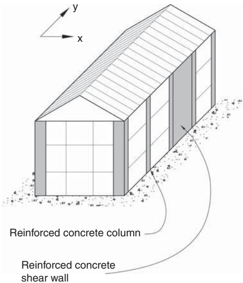
▲ 3.10 Single-storey building with x direction horizontal forces resisted by cantilever columns. Shear walls resist y direction forces.
