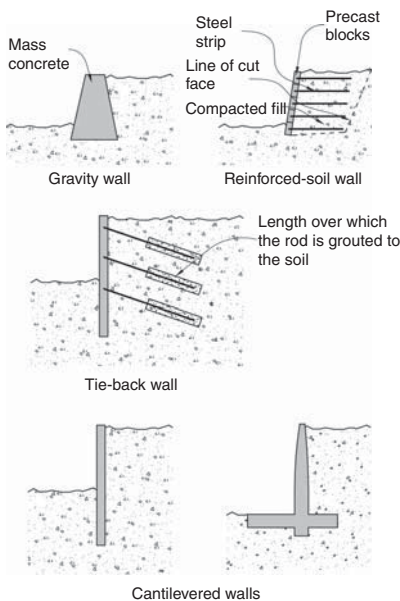
▲ 7.10 Common types of retaining structures.
