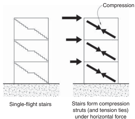
▲ 10.19 Bracing action of stairs connected to structure.
