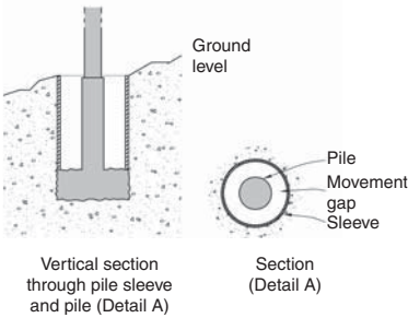
▲ 9.10 A method of avoiding a short column on a sloping site.
