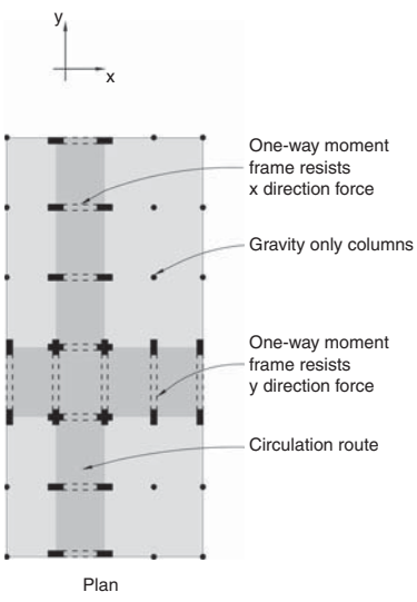
▲ 6.4 The creation of circulation routes using one-way frames whose structurally symmetrical layout does not cause torsion.
