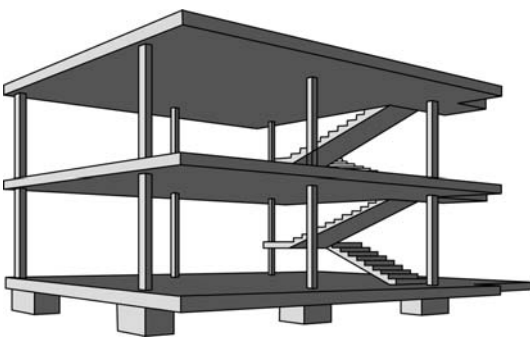
▲ 3.5 Reinforced concrete structure of the Dom-ino House, Le Corbusier, 1915.
