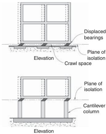
▲ 14.7 Two possible locations for an isolation plane.
