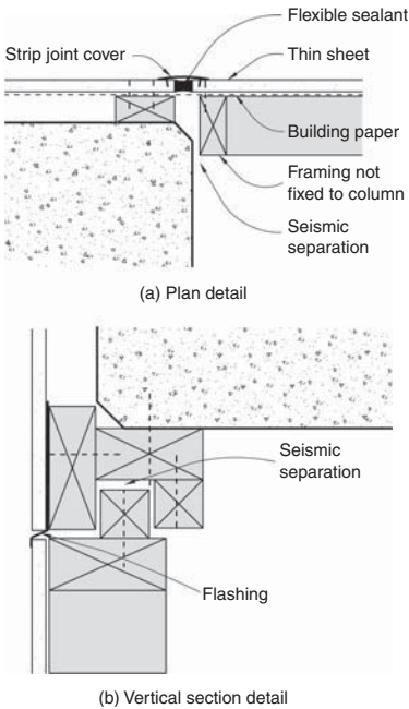
▲11.13 Separation details for thin sheet-cladding attached to a flexible structural frame.
