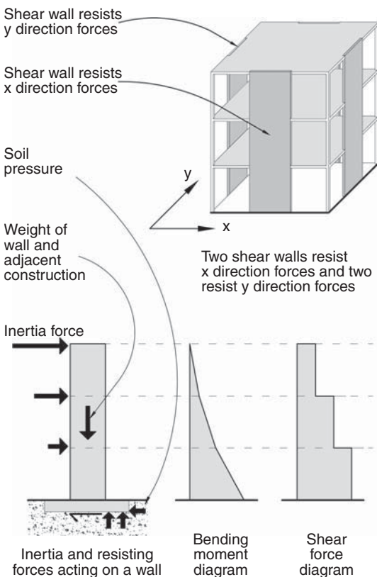
▲ 2.12 A building with shear walls resisting inertia forces in both orthogonal directions and the wall forces, bending moment and shear force diagrams.
