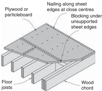
▲ 4.7 Section of a wooden floor diaphragm.
