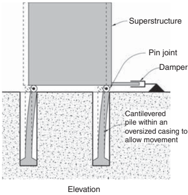
▲ 14.6 Schematic representation of an isolation system where cantilevered piles provide horizontal flexibility and centring forces.
