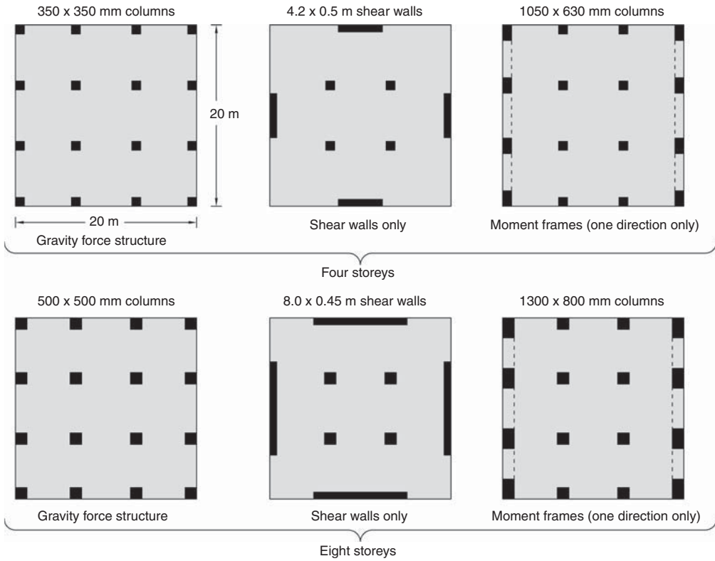
▲ 6.1 Ground floor plans of a four and an eight-storey building showing the structural footprints first for gravity forces only, and then for seismic forces where resisted by shear walls and moment frames (drawn to scale).
