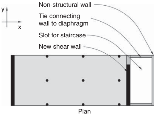
▲ 8.16 A new shear wall enables the right-hand wall to become non-structural.
