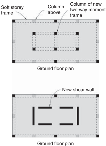
▲ 9.6 Interior moment frames or shear walls designed to resist all horizontal forces due to the unsuitability of perimeter soft storey frames.
