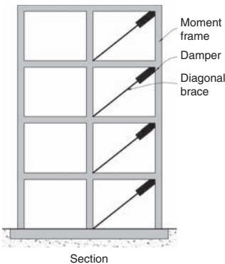
▲ 14.15 Dampers at each level of a moment frame to reduce accelerations and drifts.
