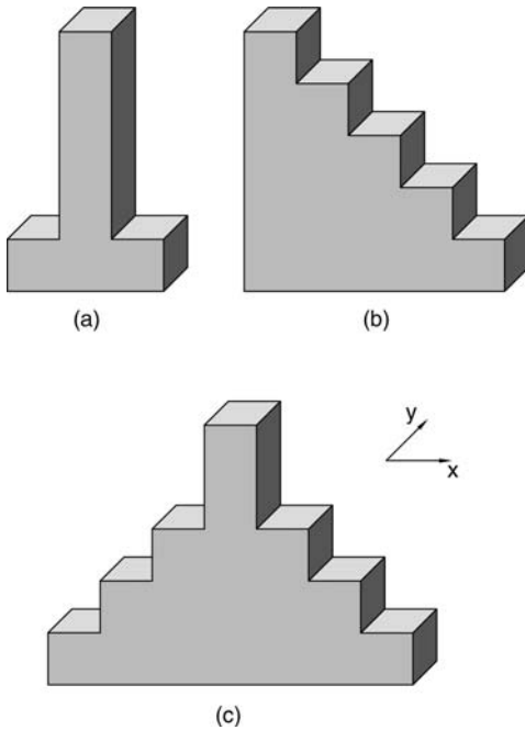
▲ 9.21 Typical setback configurations.
