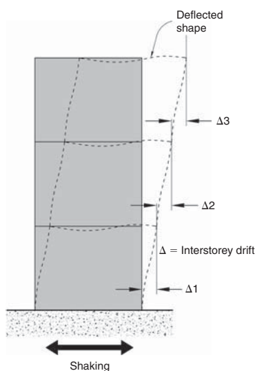
▲ 10.2 Interstorey drifts from earthquake shaking.
