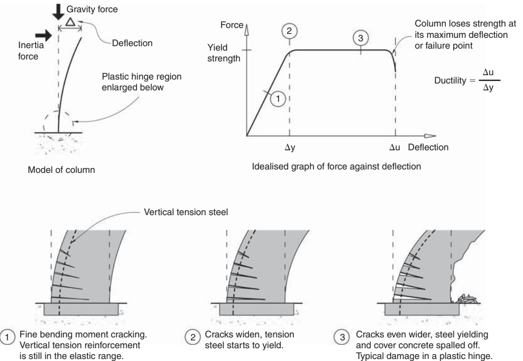
▲ 3.8 A vertical reinforced concrete cantilever column subject to a horizontal force. The force-deflection graph and the damage states reflect the ductility of the structural fuse or plastic hinge region.
