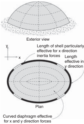
▲ 6.16 A simplified approach to understanding the horizontal resistance of a rigid shell structure.
