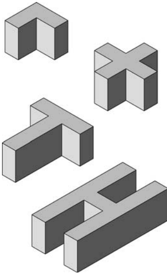
▲ 8.10 Typical re-entrant corner forms.
