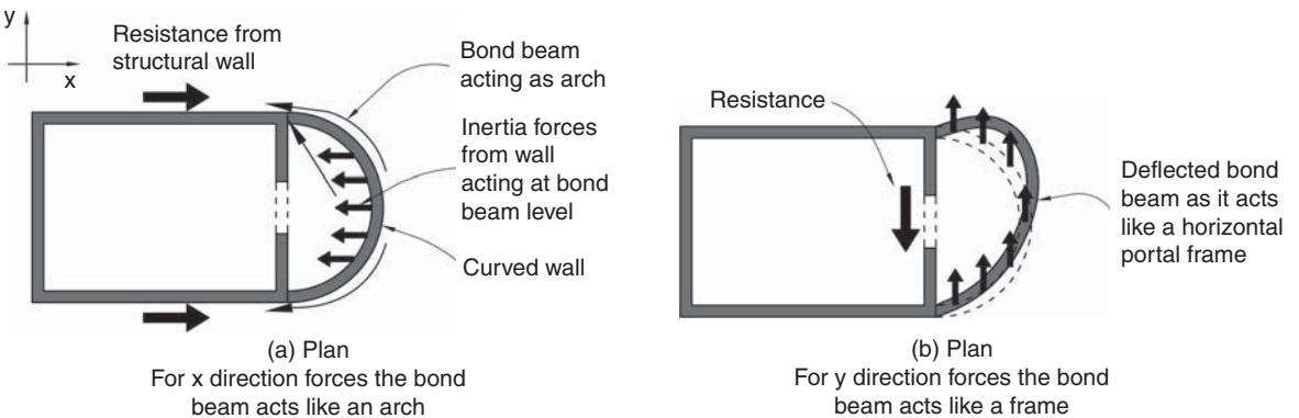
▲ 4.18 A curved bond beam behaves differently depending on the direction of horizontal force.
