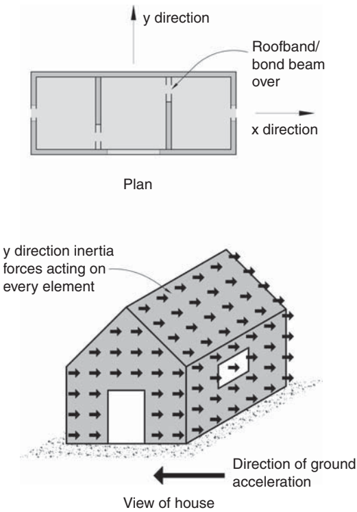
▲ 2.17 A simple building and y direction inertia forces.
