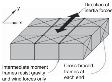
▲ 4.8 Structural layout of a single-storey light-industrial steel building.
