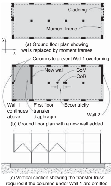
▲ 9.18 Alternatives to a discontinuous wall.
