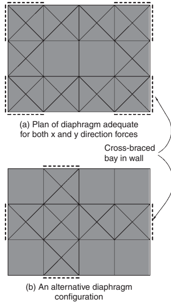
▲ 4.10 Diaphragm and wall bracing configurations suitable for both x and y direction forces.
