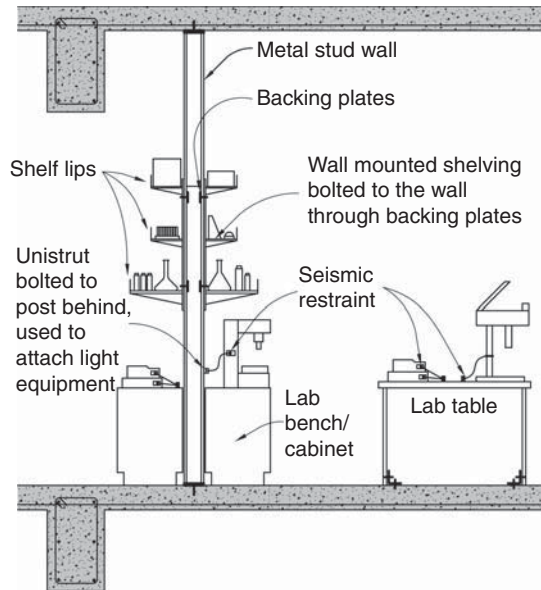
▲ 11.27 Restraints to laboratory equipment. (After Ref. 9).
