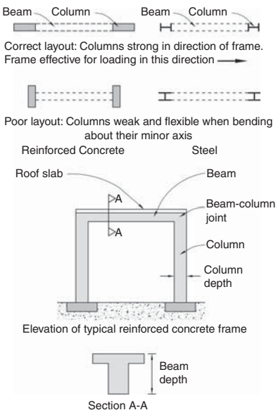
▲ 5.34 Column orientation in moment frames and frame elevation.
