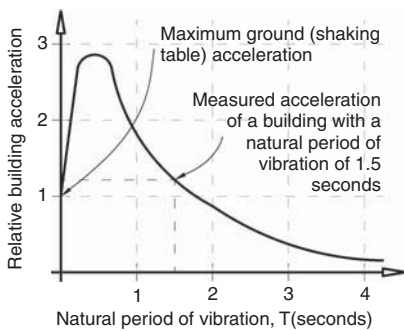
(a) Response spectrum for one earthquake record
