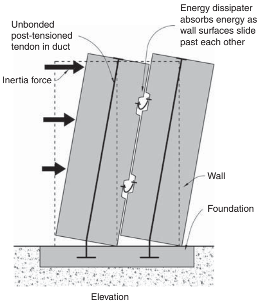
▲ 14.21 Damage avoidance precast concrete shear wall system.
