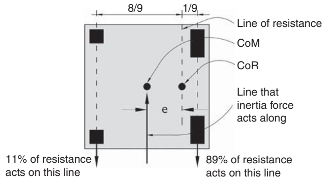
(b) Deeper right-hand columns resist more force than left-hand columns
