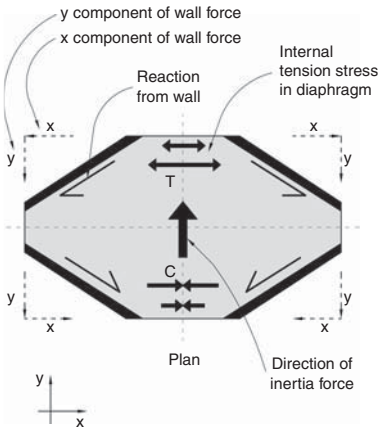
▲ 8.22 A non-parallel system showing the orthogonal force components of each wall and secondary diaphragm stresses for a y direction force.
