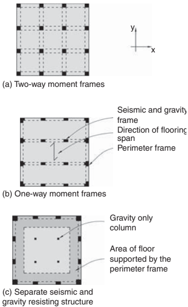
▲ 6.7 Floor plans showing different degrees of separation between seismic and gravity resisting structure.
