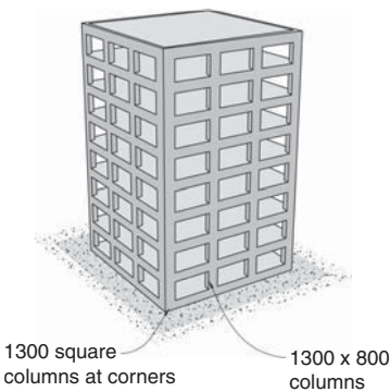
▲ 6.2 The eight-storey moment frame building of Fig. 6.1 illustrating seismic resisting structure only. Although well-configured for seismic resistance it is architecturally bland.
