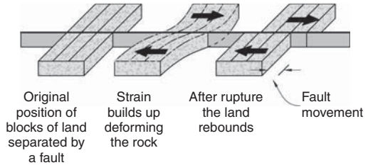
▲ 1.3 Increase of strain adjacent to a fault plane and the subsequent energy release and fault displacement.
