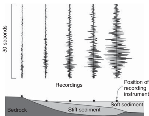
▲ 1.14 A cross-section through a geological setting near Wellington, showing acceleration records at five sites during a small earthquake. Note how the accelerations increase and frequencies reduce above deeper and soft sediments. (Reproduced with permission from J. Taber).
