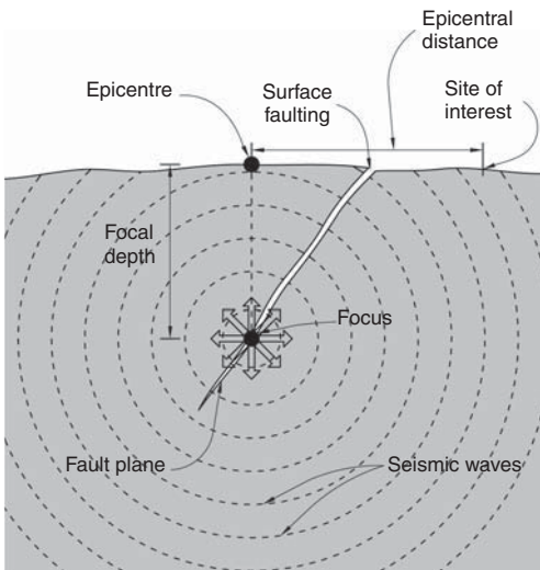
▲ 1.6 Illustration of basic earthquake terminology.
