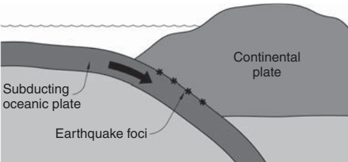
▲ 1.2 Subduction of an oceanic plate under a continental plate.
