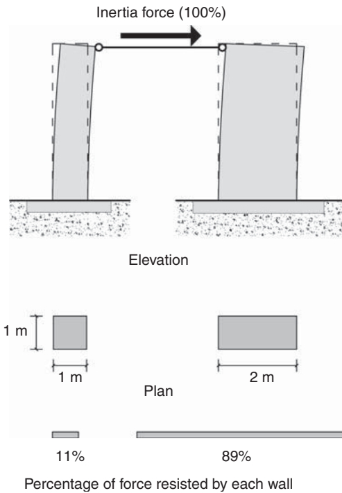
▲ 2.15 Two walls of different stiffness and the force resisted by each.
