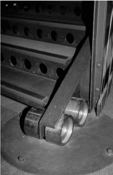
▲ 10.22 A staircase celebrating provision of interstorey drift through rollers at its base. Office building, Wellington.
