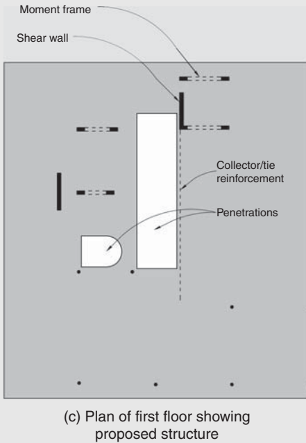
▲ 6.26 Simplified floor and roof plans of the Villa Savoye showing the proposed seismic structure if rebuilt in a seismically active area.
