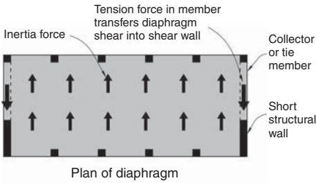
Plan of diaphragm
