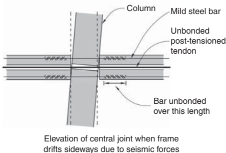
▲ 14.22 Damage avoidance detailing in a precast concrete moment frame beam-column joint.
