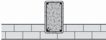
(a) Plan Reinforced concrete column provides face-load support
