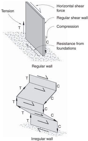
▲ 6.23 Comparison of the load path down a regular wall with that of an irregular wall at the Seattle Public Library. The additional structure required where forces change direction is not shown.
