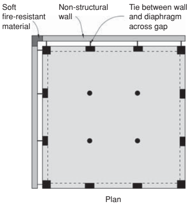
▲ 8.8 An alternative approach to achieving satisfactory configuration of a corner building by separating the strong walls from the rest of the structure and providing new moment frames to resist all seismic forces.
