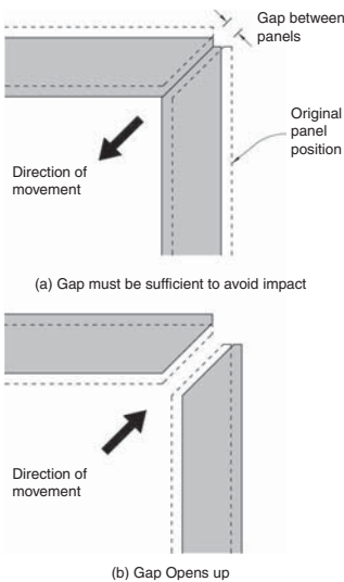
▲ 11.10 Provision for horizontal movement where panels meet at a corner as shown in plan.
