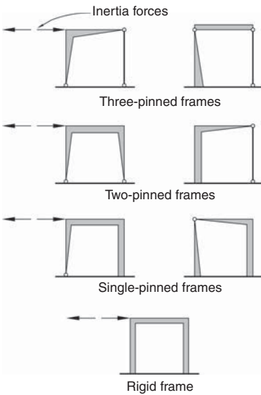
▲ 5.39 Moment frame forms with different numbers of pins. Members are detailed to partially express their bending moment diagrams under seismic forces.
