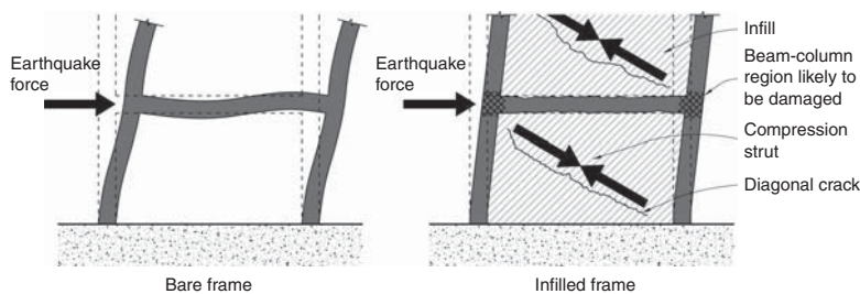
▲ 10.4 Whereas a bare frame deflects horizontally by columns and beams bending, the stiffness of a masonry infill limits horizontal movement. A diagonal compression strut forms together with a diagonal tension crack caused by elongation along the other diagonal.
