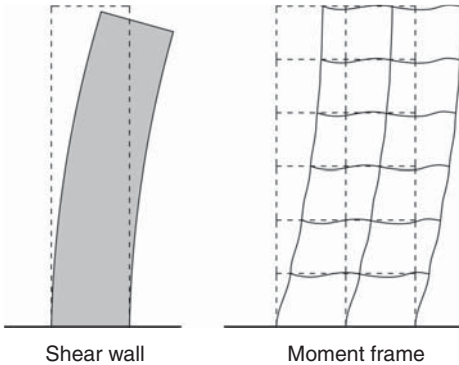
▲ 5.50 The different deflected shapes of a shear wall and a moment frame resisting seismic forces.
