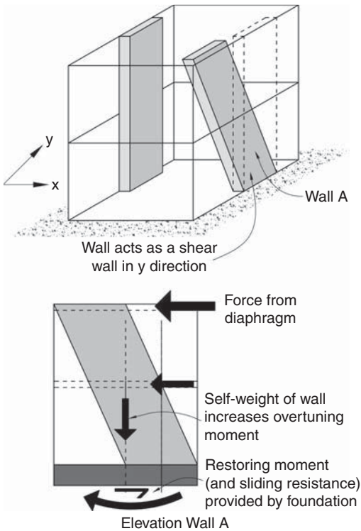
▲ 5.6 The shear wall sloping in both directions is effective in the y direction but needs support from x direction structure (not shown).
