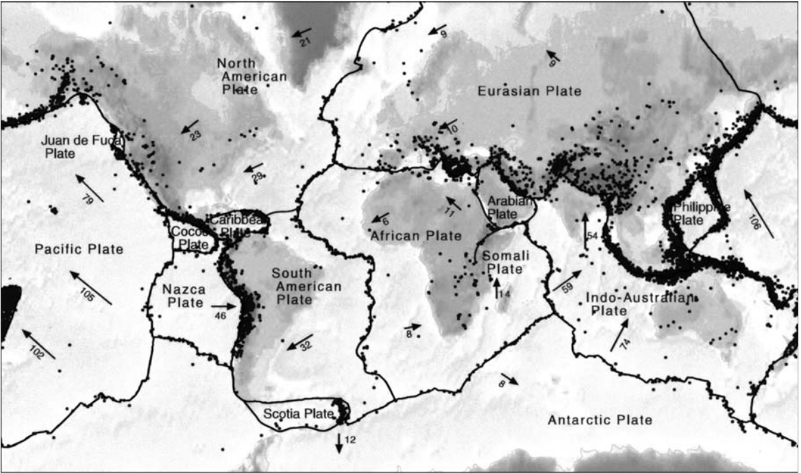
▲ 1.1 Tectonic plates and their annual movement (mm). The dots indicate positions of past earthquakes (Reproduced with permission from IRIS Consortium).
