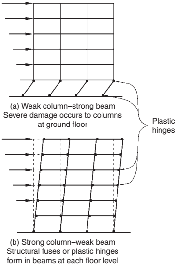
▲ 5.44 Two potential overload mechanisms of moment frames. Only the strong column–weak beam configuration is ductile.
