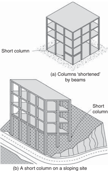
▲ 9.8 Examples of short columns among longer columns of moment frames.
