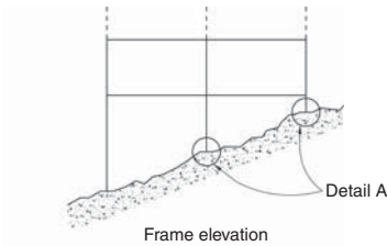
▲ 9.9 Two unequal height columns resisting seismic force.
