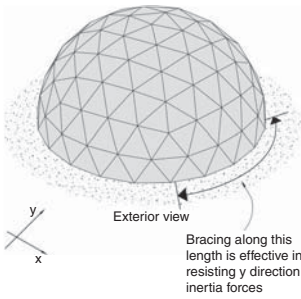
▲ 6.17 A simplified approach to a triangulated shell structure.
